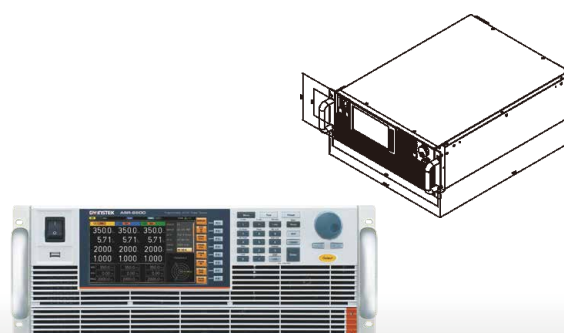
GRA-451-E Rack Mount Kit (EIA)
