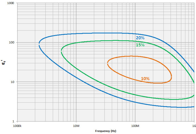
Figure 44. Permittivity (ε'ᵣ) vs. frequency (at t = 3 mm, typical)
