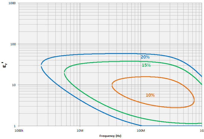
Figure 43. Permittivity (ε'ᵣ) vs. frequency (at t = 1 mm, typical)
