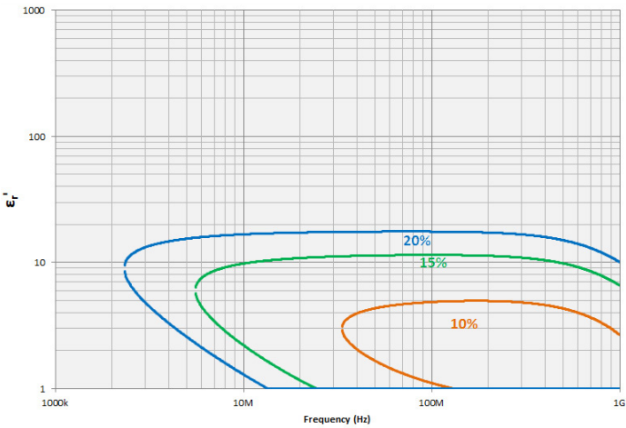
Figure 42. Permittivity (ε'ᵣ) vs. frequency (at t = 0.3 mm, typical)
